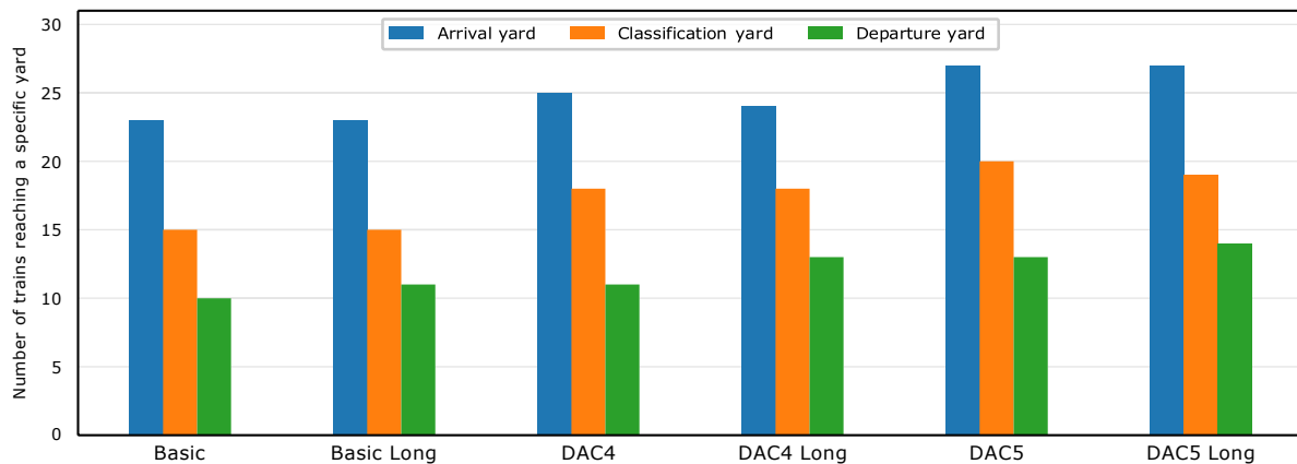
Figure 2 – Yard capacities for different scenarios after 10 hours of analysis
